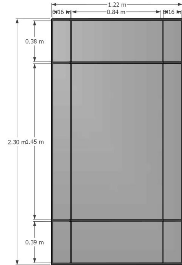
Vista frontal
